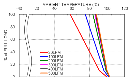
LCD30-48S05W Derating Curve With Heat-sink
